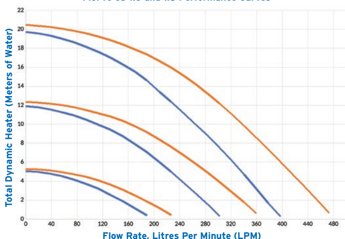
FloPro e3 1.0 and 1.5 Performance Curves
